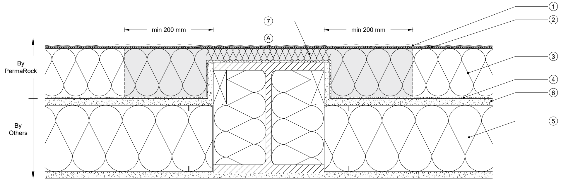
PLAN SECTION
