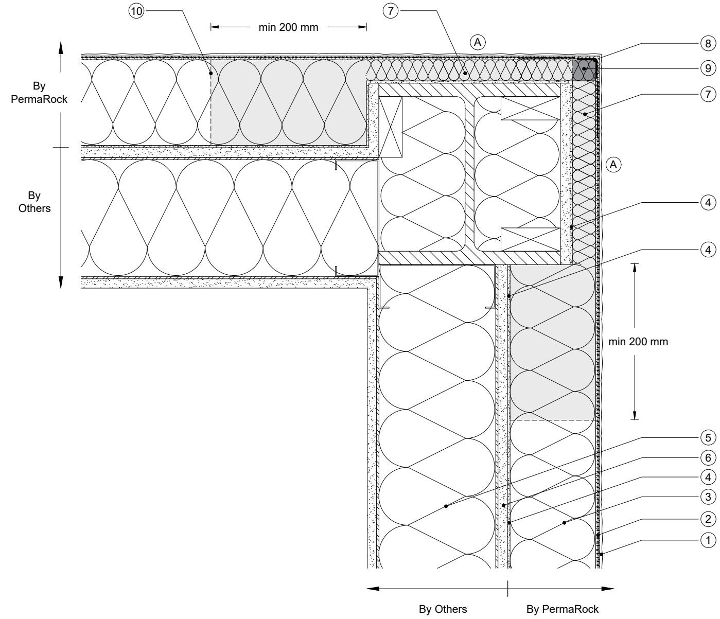
PLAN SECTION - EXTERNAL CORNER
