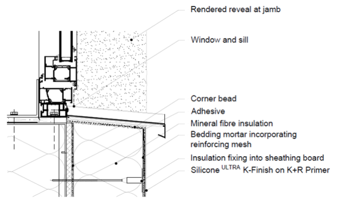
Diagram 8 - Typical cill detail
