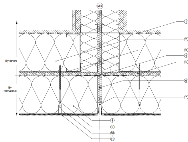
Diagram 5 - Typical vertical movement joint detail
