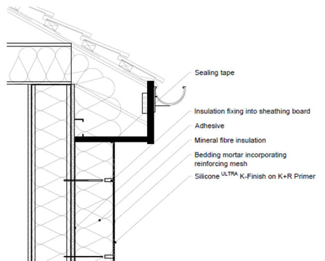
Diagram 4 - Typical overhanging eaves detail
