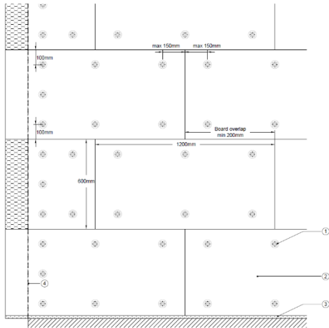
Diagram 3 - Typical fixing pattern
