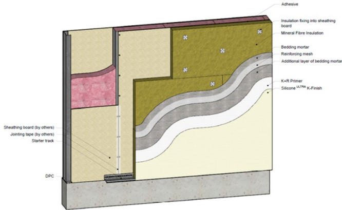
Diagram 1 - Typical build up fixed through insulation
