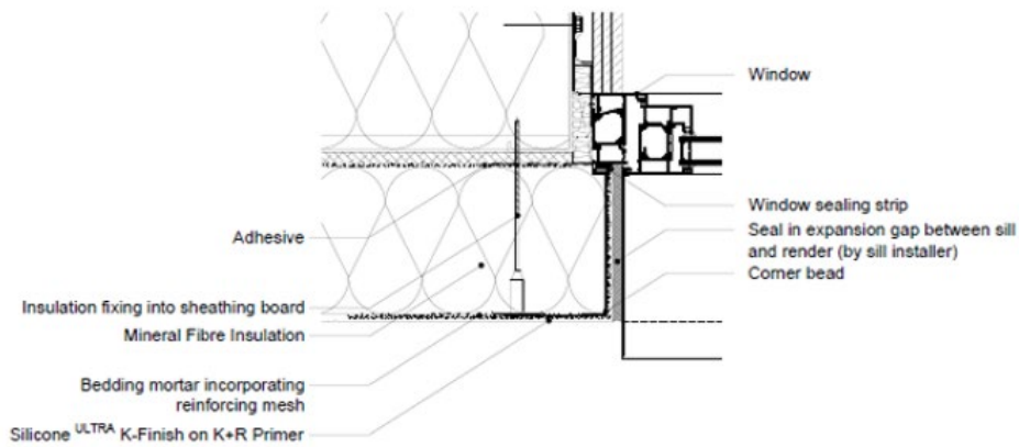
Diagram 9 - Typical window jamb detail
