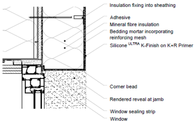
Diagram 7 - Typical window head detail
