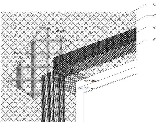
Diagram 10 - Typical opening stress patch detail
