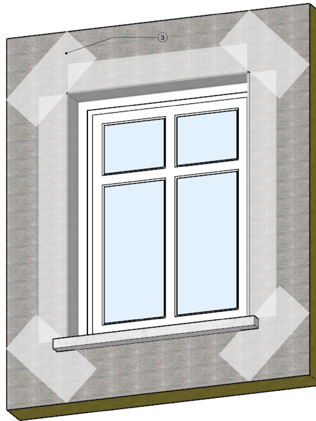
Isometric: Reinforcing Mesh into Internal Corner at Window Head/Jamb Junction
