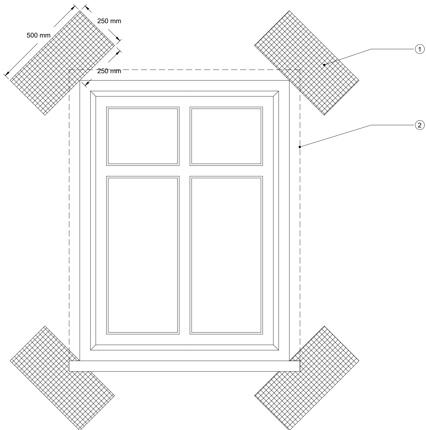
Elevation: Stress Patches at Structural Openings
