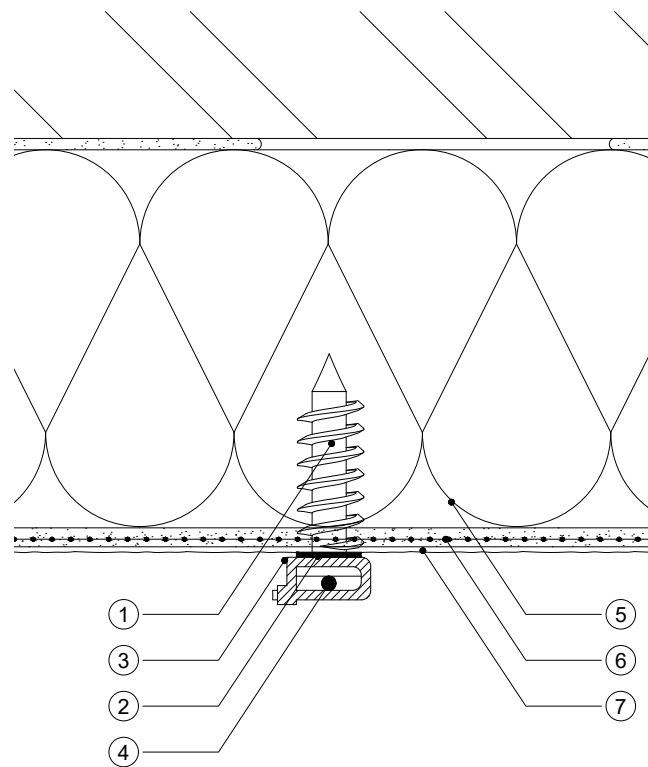
Plan Section
