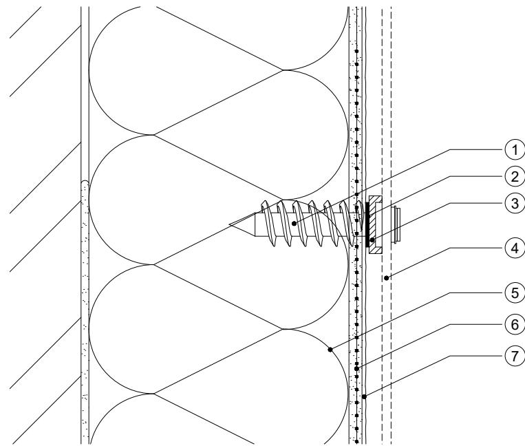
Part Section
