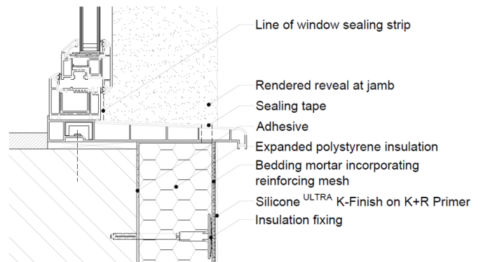
Diagram 6 - Typical cill detail
