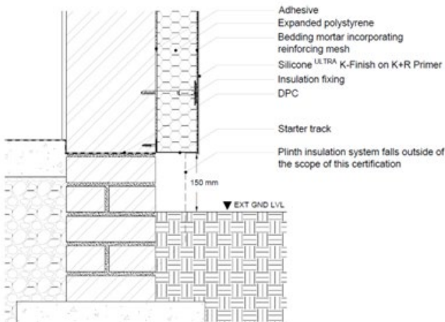
Diagram 2 - Typical standard base detail
