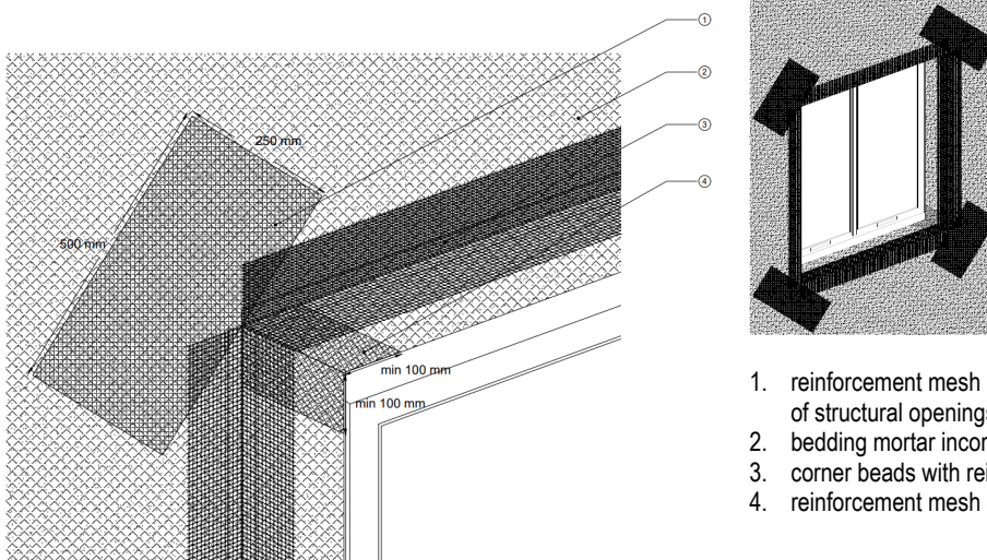
Diagram 8 - Typical opening stress patch detail
