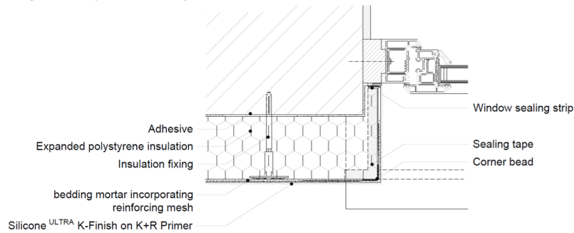
Diagram 7 - Typical window jamb detail
