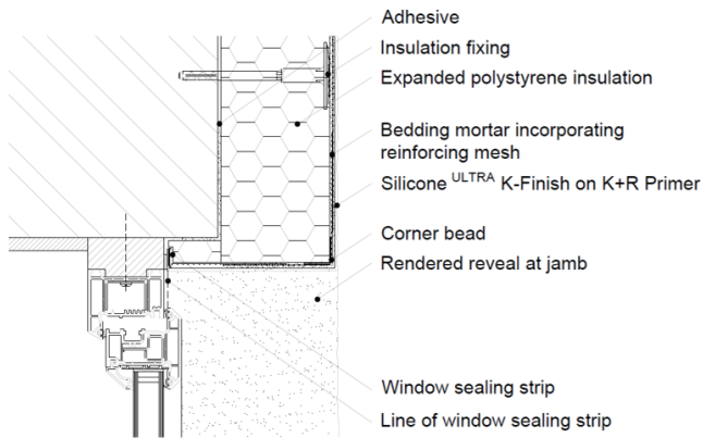
Diagram 5 - Typical window head detail
