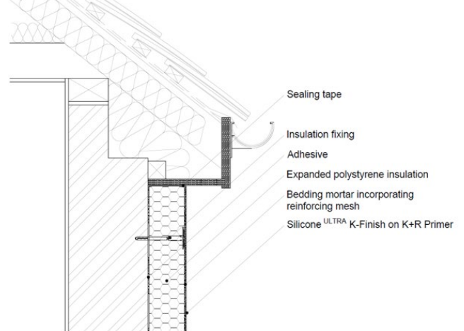
Diagram 3 - Typical overhanging eaves detail
