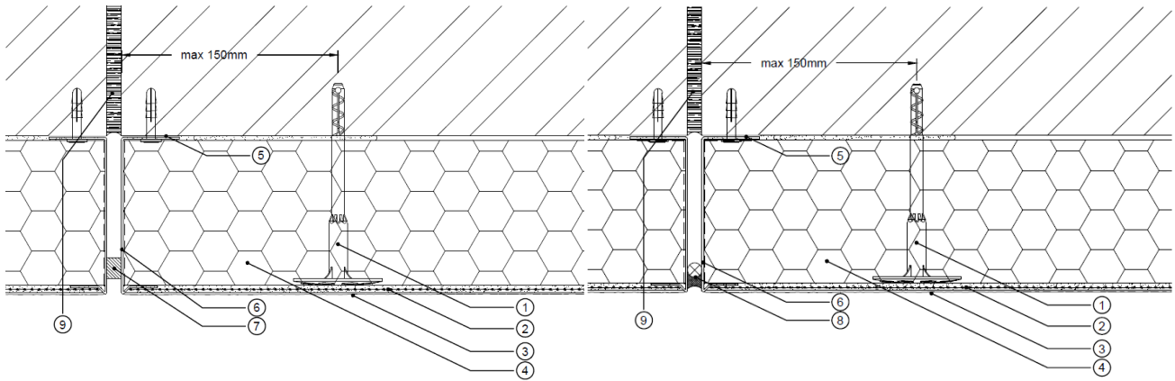
Diagram 4 - Typical vertical movement joint detail with joint tape or mastic seal
