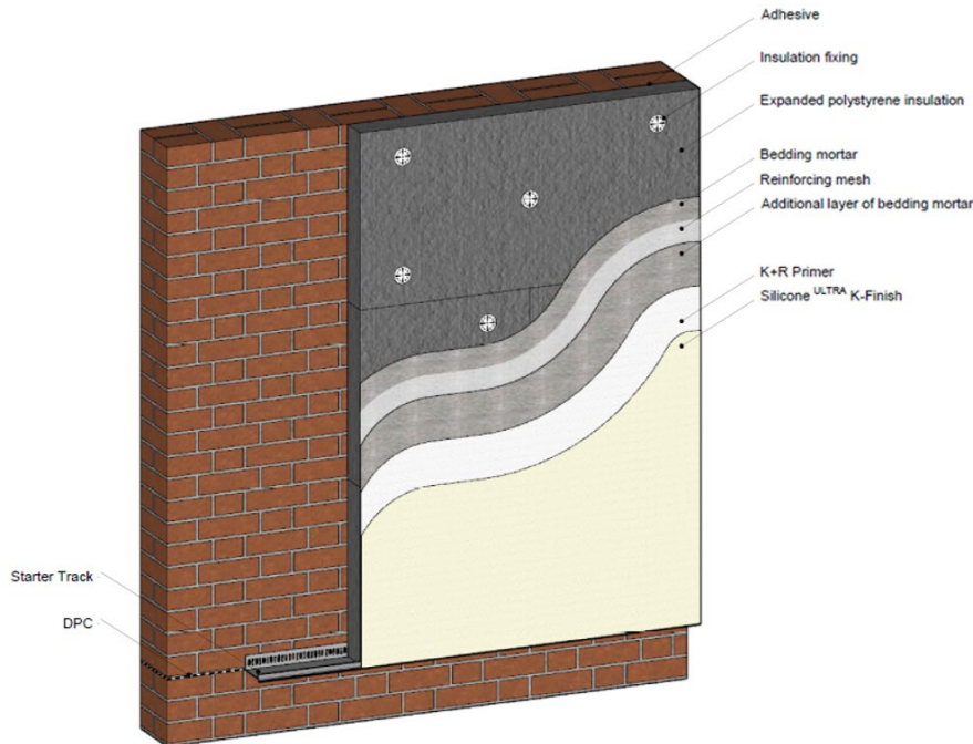
Diagram 2 - Typical standard base detail
