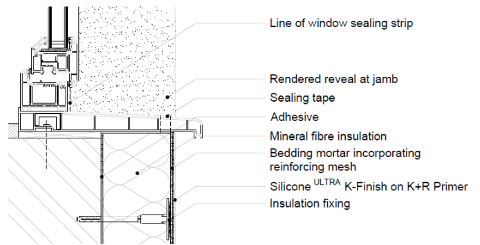
Diagram 8 - Typical cill detail
